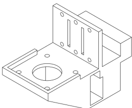
Gripper Carriage Body
