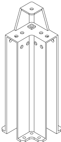
Idler Pulley Housing
