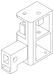
Linear Carriage Body Left
