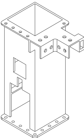
CoreXY Motor Mount Left
