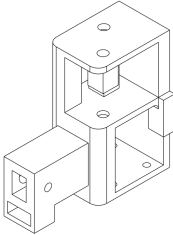
Linear Carriage Body Right
